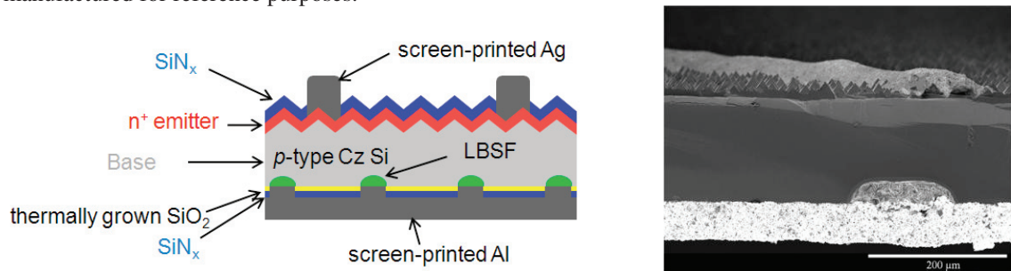
Fig. 3: Schematic (left) and SEM image (right) of a PERC solar cell with screen-printed front and rear contacts with SiO 2 / SiN x rear passivation. Note that the breaking edge in the SEM image is not perpendicular to the contact line direction at the front and the rear.
